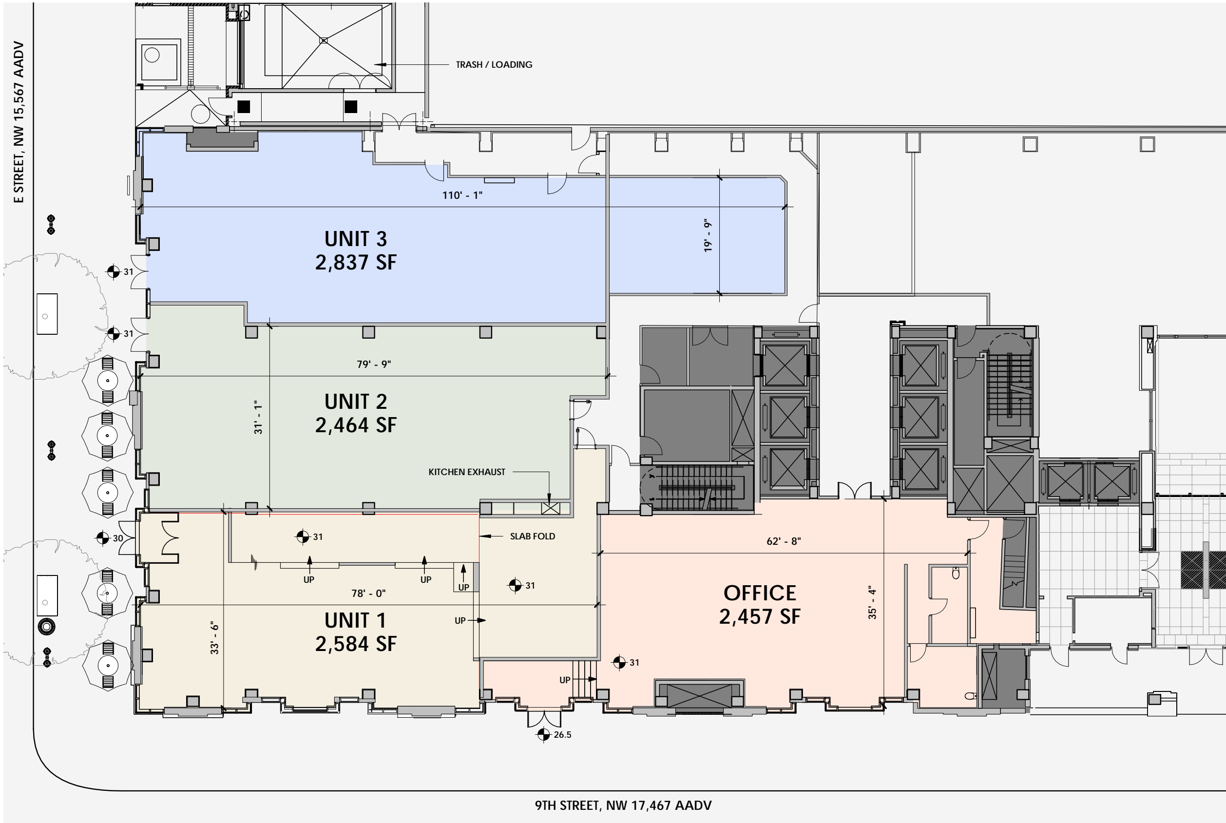
LEVEL L2 PLAN
